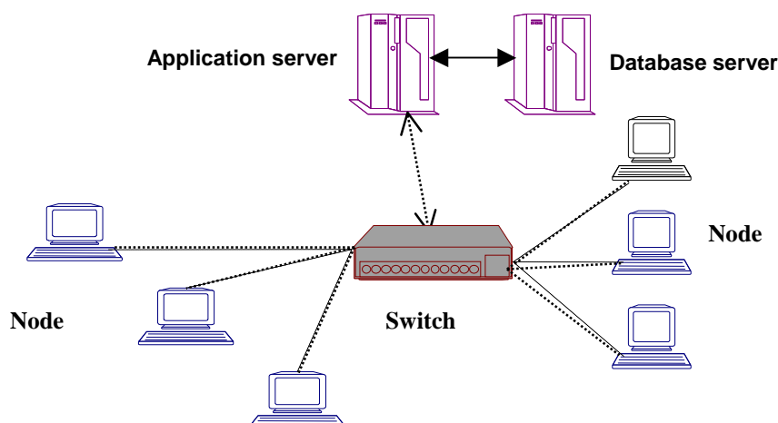
Three-tier architecture
